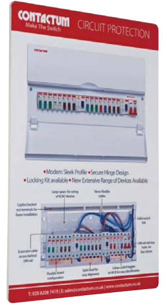
Consumer Unit
